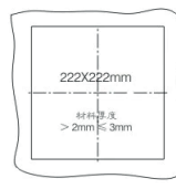
mounting dimension
