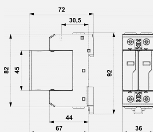
Dimension drawing
