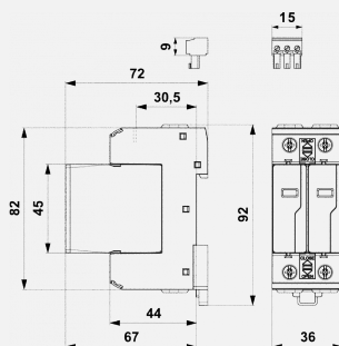
Dimension drawing
