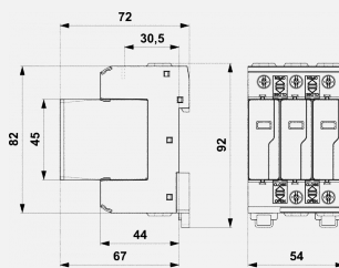
Dimension drawing
