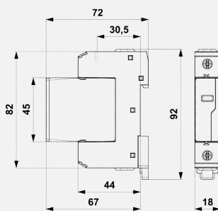
Dimension drawing
