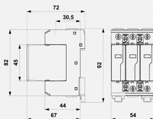
Dimension drawing
